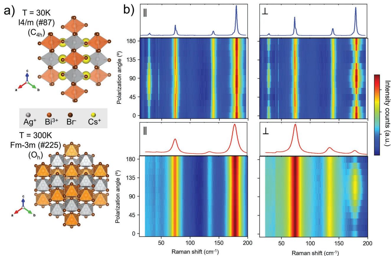
Figure 3. a) Crystal structures of the 3D \text{Cs}_2\text{AgBiBr}_6 PSK drawn using VESTA software [44] for the low- and high-temperature phases [26] from the perspective of the (111) plane that is exposed in the experiment. b) Color plots of the angle dependence of the Raman spectrum for polarized (||) and depolarized ( \perp ) configurations. The integrated Raman spectra along the polarization angle are shown on top of the color plots.
