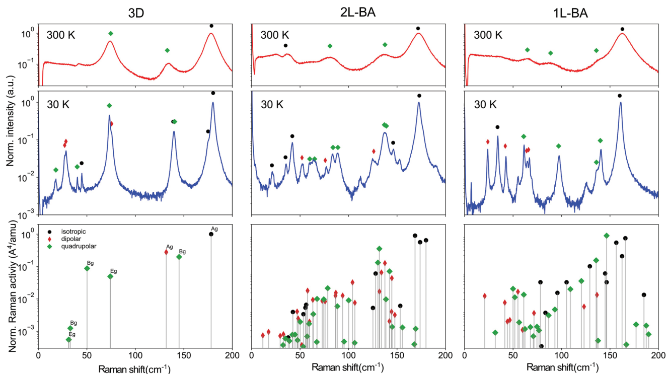
Figure 2. Comparison of the experimental Raman spectra using y-axis logarithmic scale for highlighting the low-intensity modes and DFT results for 3D, 2L-BA, and 1L-BA samples. Experimental data are unpolarized spectra measured at RT and 30 K (shown on semi-log scale), normalized to the strongest peak. The DFT modeling results are displayed in terms of Raman frequency and activity. The symbols mark the polarization of the modes that are defined by the depolarization factor D , classified as “isotropic” for D < 0.15 (black circles), “dipolar” for 0.15 < D < 0.72 (red diamonds), and “quadrupolar” for D > 0.72 (green diamonds).
