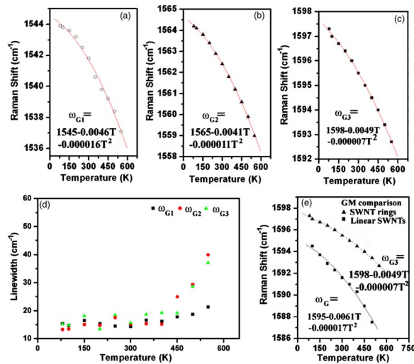
FIG. 3. (Color online) (a)–(c) G modes frequencies shift as a function of temperature for the SWCNT rings. The solid lines are the fits with second-order formula. (d) Linewidth dependence of the G peaks on the temperature for the SWCNT rings. (e) The comparison of the temperature-induced GM frequency variations between the SWCNT rings and the linear SWCNTs.
